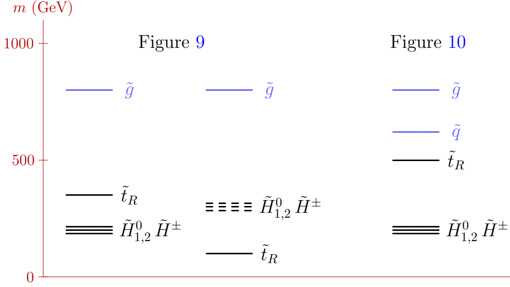
Figure 8: Mass spectra of the models studied in this section. The label \tilde{q} indicates the four second-generation squarks ( \tilde{c}_R , \tilde{s}_R , \tilde{c}_L , \tilde{s}_L ). The LSP decays to jets via RPV in all cases. Dashed lines indicate particles that do not participate in the dominant gluino decay processes. Blue lines indicate masses that we will vary.
