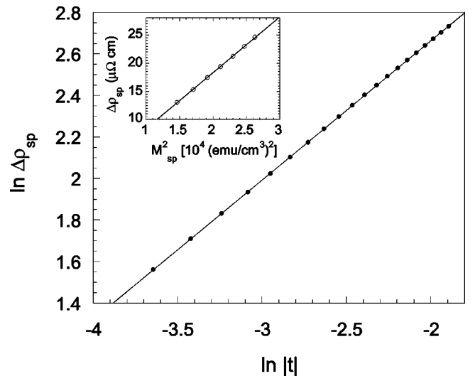
FIG. 2. Critical behavior of \Delta\rho_{sp} with respect to the reduced temperature t=(T-T_c)/T_c from 130 to 149 K with T_c=153 K. A linear fit is shown. The inset shows the correspondence between \Delta\rho_{sp} and the square of the measured spontaneous magnetization M_{sp} .
