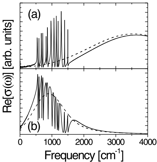
FIG. 4. Calculated PA spectra (solid lines) using the CDW response function f(\omega) (broken lines) with onset 2\Delta at (a) 2\Delta = 3600 \text{ cm}^{-1} and FWHM of 2400 \text{ cm}^{-1} , (b) 2\Delta = 800 \text{ cm}^{-1} and FWHM of 800 \text{ cm}^{-1} .
