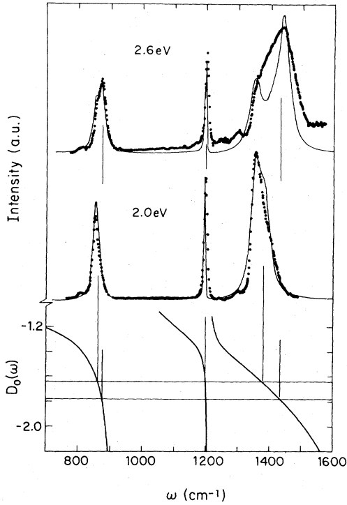
FIG. 2. As in Fig. 1, but for (\text{CD})_x .
