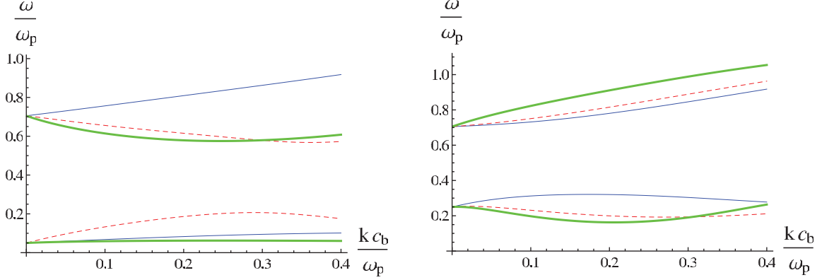
Fig. 1: (Colour on-line) Left: surface plasmon dispersion relation \omega(k) for different values of the surface scattering parameter \alpha in eq. (17): \alpha = 0.1 (thin blue lines), \alpha = 1 (dashed red lines) and \alpha = 10 (thick green lines). Upper lines starting at \omega_p/\sqrt{2} : real part; lower lines: imaginary part \times(-1) . Other parameters: \omega_s = 0 , c_s/c_b = 1 , \omega_p\tau = 10 , \omega_p\tau_s = 10 , \tau' = \infty and \tilde{d} = \omega_p d/c_b = 3.5 . Right: effects of a nonzero restoring force in the surface layer (plasma frequency \omega_s ): \omega_s = 0 (thin blue curves), \omega_s/\omega_p = 0.5 (dashed red curves) and \omega_s/\omega_p = 0.9 (thick green curves). The upper curves are the real part and the lower ones are the imaginary part \times(-5) . The other parameters are c_s/c_b = \sqrt{3} , \omega_p\tau = 10 , \omega_p\tau_s = 10 , \tau'\omega_p = 1 , \alpha = 0.1 and \tilde{d} = 7 .
